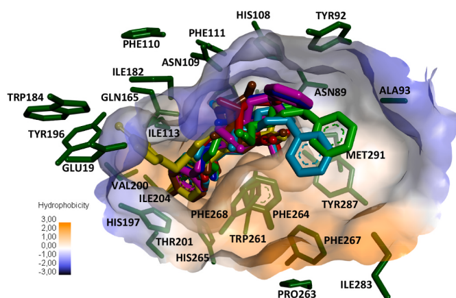
Fig. 3. Binding site residues of NK1R (dark green), hydrophobicity surface and best docked poses for: 8α (magenta), 8β (green), 9α (red), 9β (brown), 10α (dark blue), 10β (bright blue) and Aprepitant (yellow). For clarity, hydrogen atoms have been removed. Orange colour represents the most hydrophobic surface area; blue colour represents the least hydrophobic.
