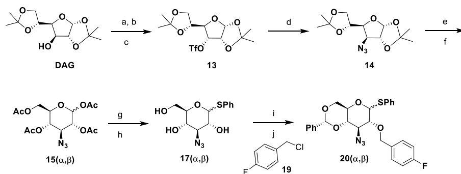
Scheme 1. Synthesis of p -fluorobenzyl D-glucose derivative 20(α,β) . Reagents and conditions: (a) P_2O_5 , dimethylsulfoxide (DMSO), 50 °C; (b) NaBH_4 , H_2O , tert -butyl methyl ether (TBME), 0 °C–10 °C; (c) Tf_2O , CH_2Cl_2 : pyridine (10:1), 0 °C (quant. yield); (d) NaN_3 , dimethylformamide (DMF), rt (quant. yield); (e) CF_3COOH:H_2O (20:3), 0 °C; (f) Ac_2O , pyridine, rt, \alpha:\beta 1:0.7 (74% yield); (g) Ph-SH , BF_3 \cdot Et_2O , CH_2Cl_2 , 40 °C, \alpha:\beta 0.2:1; (h) NaOCH_3 , MeOH, rt, \alpha:\beta 0.1:1 (77% yield); (i) PhCH(OCH_3)_2 , 10-camforsulfonic acid (CSA), DMF, rotavapor, 35 °C, \alpha:\beta 1:10; (j) NaH , NB_{u_4} , 19 , THF, rt, \alpha:\beta 1:10 (quant. yield).
