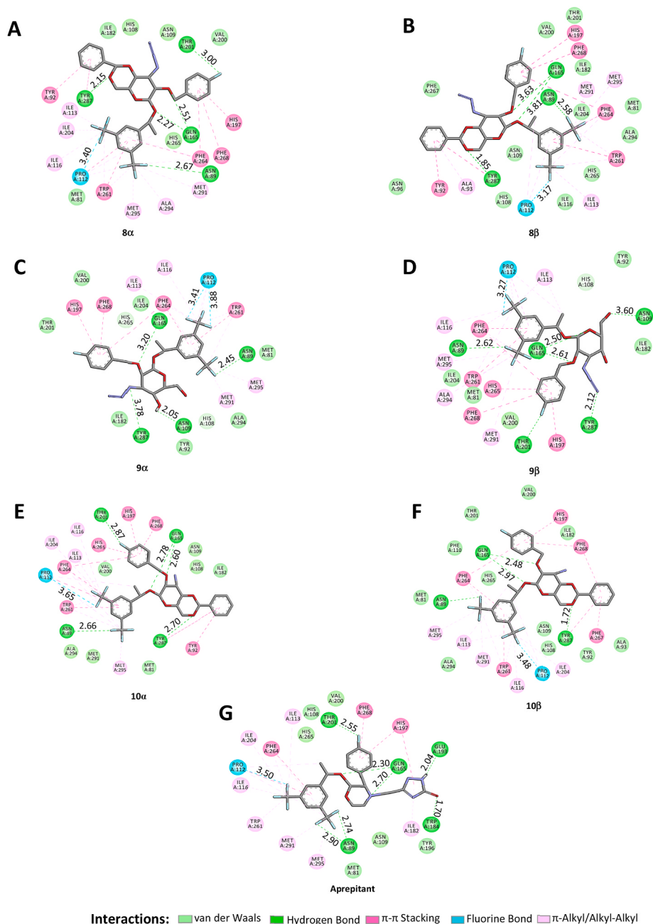
Fig. 2. Two-dimensional view of the interaction type for the best docked poses of 8α (A), 8β (B), 9α (C), 9β (D), 10α (E) 10β (F) and Aprepitant (G) with surrounding amino acids of NK1R (PDB ID: 6HLO). The distances for hydrogen bonds and fluorine bonds are given in Å.
