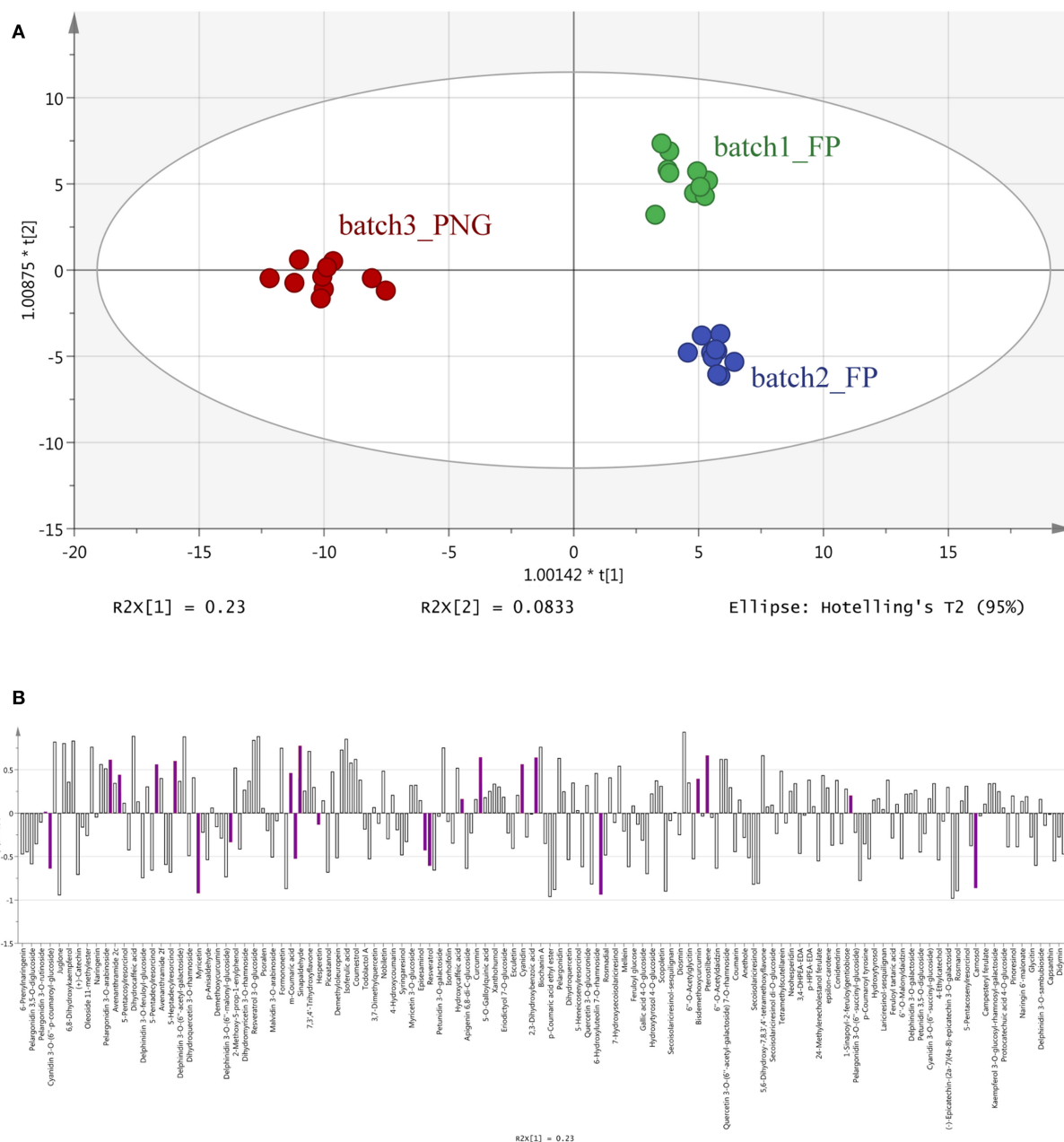
FIGURE 2 | Orthogonal Projections to Latent Structures Discriminant Analysis (OPLS-DA) on vanilla sample phenolic profiles. Individual replications are given in the model score plot (A) , whereas loadings column plot is reported in the (B) . Compounds selected by VIP analysis are reported in color in the loadings column plot. PNG samples (red samples) are clustered on the left whereas Tahitian samples (green and blue samples) on the right side of the plot. Both geographic origin and cultivars were responsible for the actual phenolic signature of the samples.
