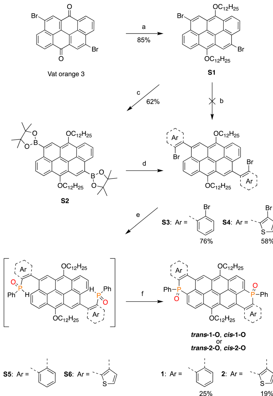
Scheme 1 Synthetic routes toward 1-O, and 2-O as mixtures of cis & trans isomers. (a) Dodecyl bromide, sodium dithionite, 0.1 M NaOH, 70 °C, 3 h. (b) K_2CO_3 , 3-bromo-2-borapinacolatothiophene, Pd(PPh_3)_4 , 1,4-dioxane, 100 °C, 20 h. (c) (Bpin)_2 , Pd(dppf)Cl_2 , KOAc, dioxane, 100 °C, 20 h. (d) 2,3-Dibromothiophene (or 1,2-dibromobenzene), Pd(PPh_3)_4 , K_2CO_3 , Dioxane/ H_2O : 3 : 1, 100 °C, 20 h. (e) 1: n -BuLi, PhPCl_2 , THF, −78 °C, 4 h; 2: H_2O , 1 h. (f) AgNO_3 , CH_3CN /Toluene: 1 : 1, 90 °C, 12 h.
