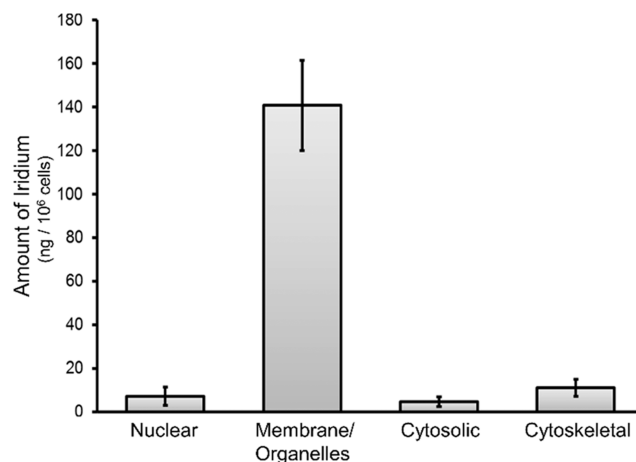
Figure 6. Subcellular distribution of complex 6 . The nuclear, membrane/organelles, cytosolic, and cytoskeletal fractions of A549 cells treated for 4 h with complex 6 at 10 \mu M were isolated, and the iridium content in each fraction was measured by ICP-MS. The mean values and standard deviation obtained in two independent experiments are shown.
