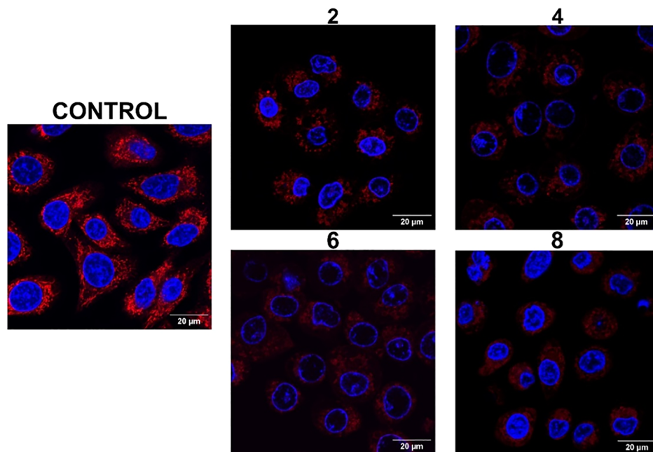
Figure 8. Effect of the photoactivated complexes on mitochondria. A549 cells were incubated with complexes 2, 4, 6, and 8 for 4 h at the corresponding IC 50,light followed by photoactivation with a blue light (1 h, 460 nm, 24.1 J cm -2 ) or incubated with medium alone as a control. Mitochondria were stained with MitoTracker Red CMX and visualized in red (λ ex = 554 nm; λ em = 576 nm) by confocal microscopy. Nuclei of living cells were counterstained with Hoechst 33342 (λ ex = 350 nm; λ em = 461 nm) and visualized in blue.
