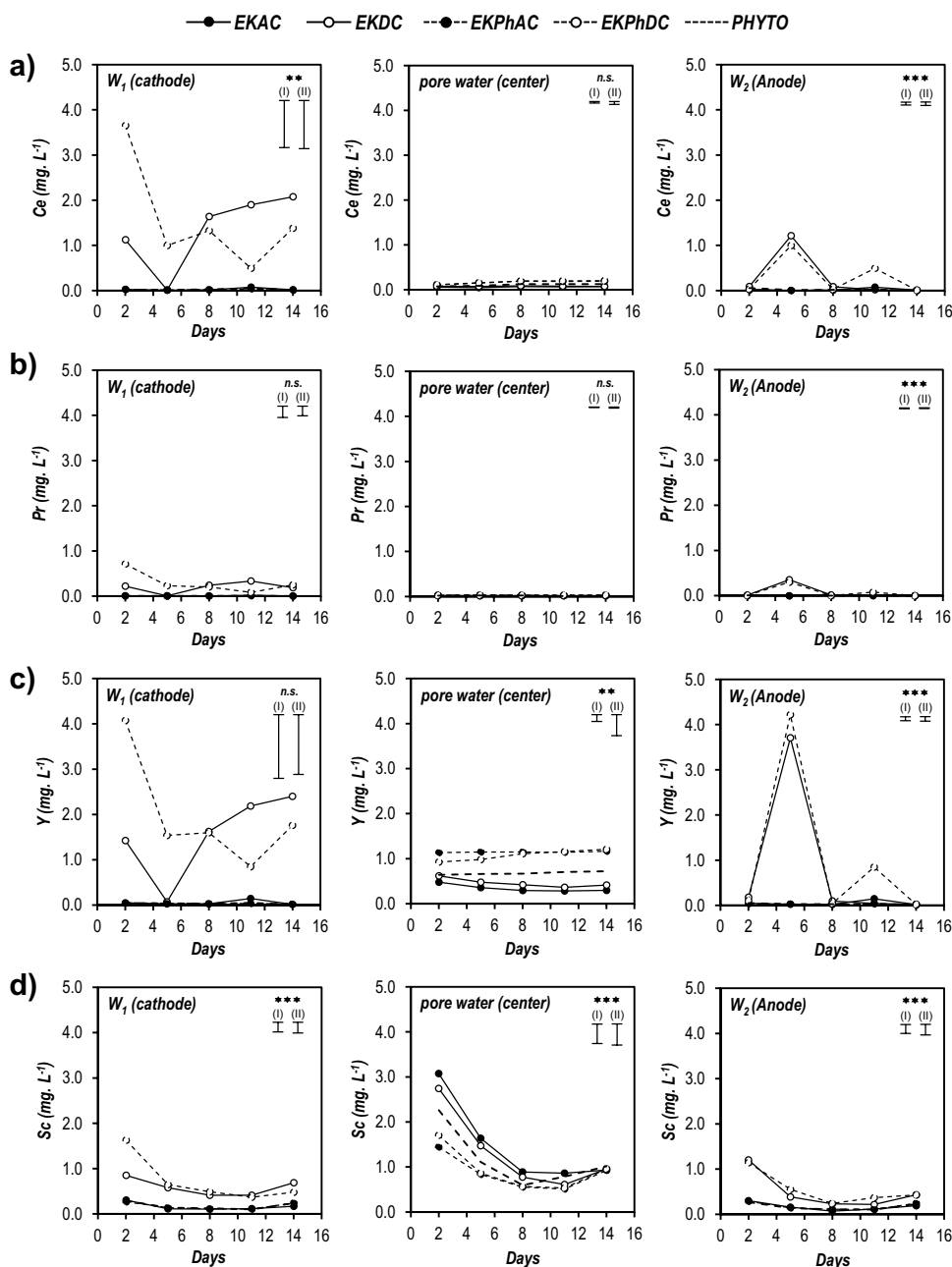
Fig. 3 REEs concentrations (mg L -1 ) in the water obtained from electrode wells (W 1 and W 2 ) and the soil pores (collected from the middle section of each container by Rhizon samplers) sampled (n = 3) just before turning off the electric current on different days: a Ce; b Pr; c Y; d Sc. Treatments applied: PHYTO: plants and no electricity; EKDC and EKAC: electric current and no plants; EKPhDC and EKPhAC: plants and electric current. For each REE and section, single, double, and triple asterisks indicate significant level (two-way ANOVA analysis) of “concentration × time” interaction. Vertical bars show LSD test (p ≤ 0.05): (I) for same level of EK/Phyto treatment and (II) for different levels of treatments
