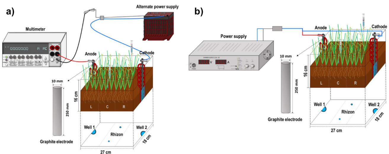
Fig. 1 Schematic representation of the experimental setup used in the electrokinetic-assisted phytoextraction tests: a alternate current treatments; b direct current treatments
