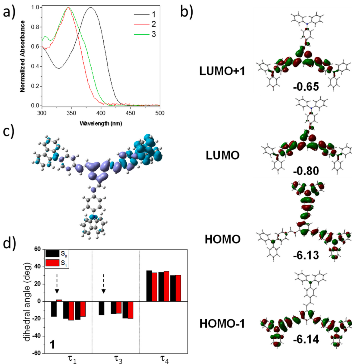
Fig. 2. (a) Normalized absorption spectra of compounds 1–3 in dichloromethane solution (sample concentrations were 1 \mu M) [2]. (b) Isocontour plots (0.02 au) of some selected frontier molecular orbitals of 1 (and their energy levels in eV) in dichloromethane solution computed at the M06-2X/6-31G* level of theory. (c) Charge density distribution (hole in green; electron in purple) calculated for 1 in S_1 state (TD-M06-2X/6-31G*, dichloromethane solution). (d) Some selected dihedral angles ( \tau_1 , \tau_2 and \tau_4 of each branch of the molecule) calculated for the S_0 and S_1 states of 1 in dichloromethane (the arrows indicate significant changes). (For interpretation of the references to color in this figure legend, the reader is referred to the Web version of this article.)
