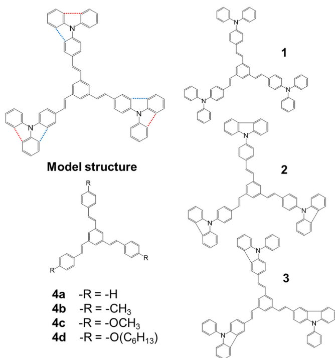
Scheme 1. Chemical structure of molecules 1–3 along with some related compounds ( 4a , 4b and 4c ). Model structure shows the interrering C–C bonds that differentiate the studied molecules.
