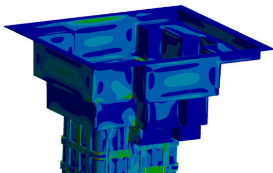
Fig. 8. #46 Candidate, Variant 1–30 mm thick top segment deformation.
