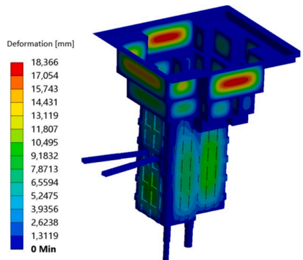
Fig. 9. #46 Candidate, Variant 2 – total.
