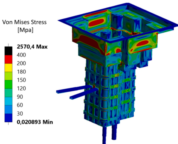
Fig. 6. #46 Candidate, Variant 1 – Equivalent Stress Field.
