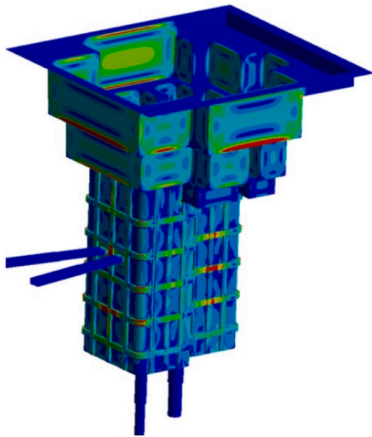
Fig. 11. #53 Candidate, Variant 2 – Stress Field.
