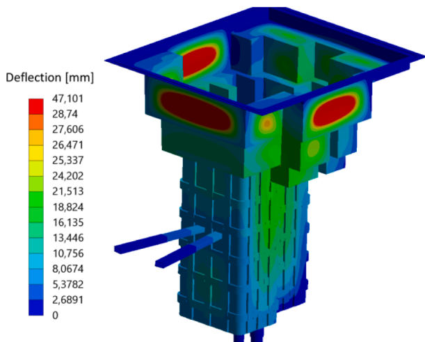
Fig. 4. #46 Candidate, Variant 1 – total deformation.
