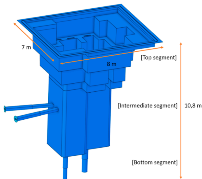
Fig. 1. Test Cell Liner main dimensions.
