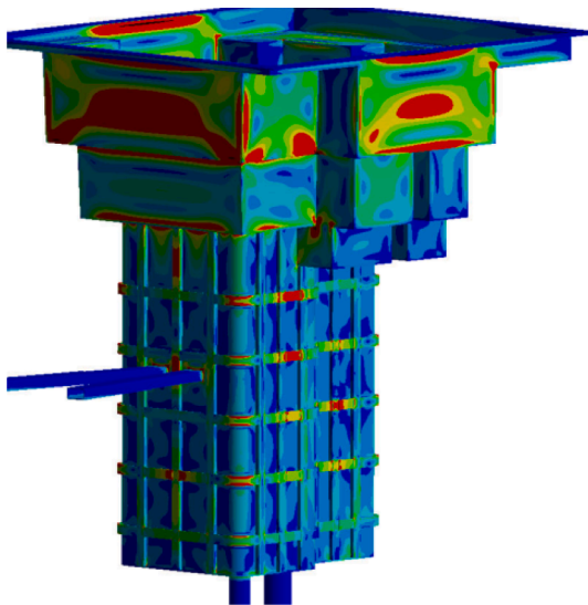
Fig. 7. #53 Candidate, Variant 1 – Equivalent Stress Field.
