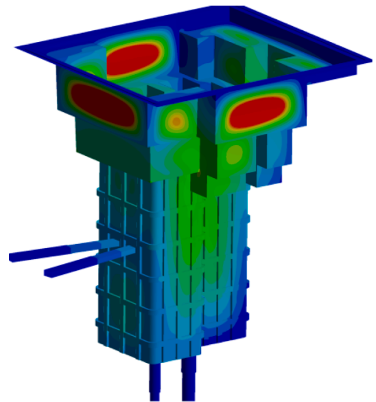
Fig. 5. #53 Candidate, Variant 1 – total deformation (same coloring as before).
