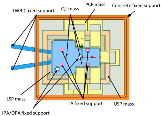
Fig. 3. Fixations and applied masses.
