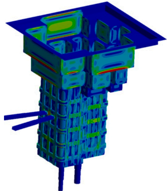
Fig. 10. #46 Candidate, Variant 2 – Stress Field.
