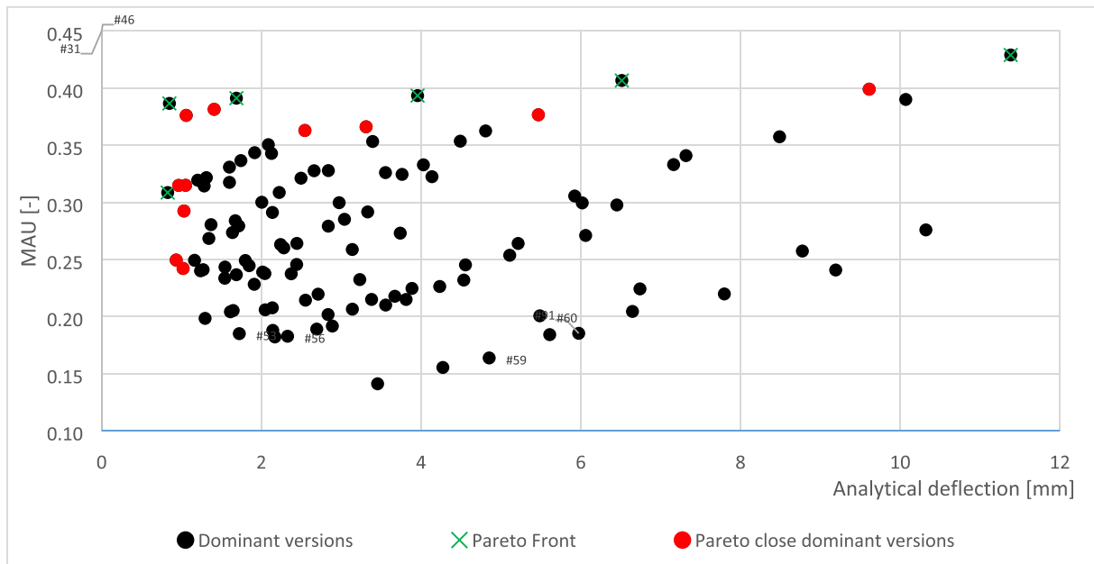
Fig. 2. Tradespace analysis of candidate stiffener profiles.
