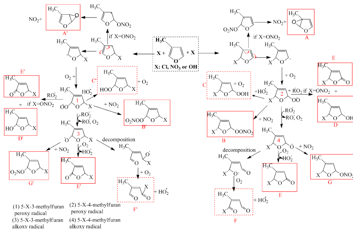
Scheme 1. Reaction sequences of 3-methylfuran and X radical initiated by an addition process: possible mechanism for the formation of 5-X-3-methyl-2(5H)-furanone and 5-X-4-methyl-2(5H)-furanone. X: Cl, OH or NO 3 . Compounds C/C' and F/F' were not detected.
