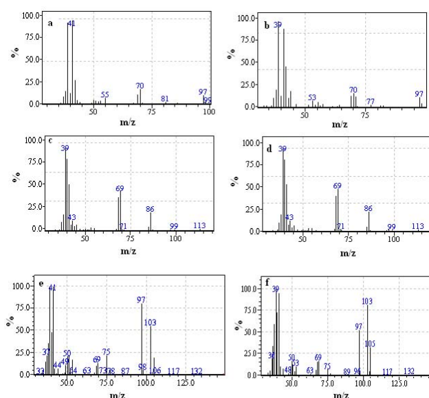
Fig. 2. (a) Experimental electron impact mass spectra (EI-MS) of peaks F (tr = 11.4 min) and G (tr = 11.8 min). (b) Experimental electron impact mass spectra (EI-MS) of the 2-methylbutenedial synthesized. (c) Experimental electron impact mass spectra (EI-MS) of peak L (tr = 28.2 min). (d) Experimental electron impact mass spectra (EI-MS) of the commercial 5-hydroxy-4-methyl-2(5 H )-furanone. (e, f) Mass spectra by electron impact ionization (EI) of peaks J and K assigned to a molecular formula C 5 H 5 O 2 Cl.
