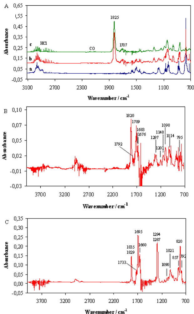
Fig. 4. Experimental infrared absorption spectra from the reaction of: (A) 3-methylfuran with chlorine atoms (a) before photolysis, (b) after 15 min of photolysis (c) residual spectrum from b after subtraction of 3-methylfuran, H 2 O with the CO 2 absorption zeroed; (B) 3-methylfuran with hydroxyl radical (residual spectrum of products after 8 min of reaction), (C) 3-methylfuran with nitrate radicals (residual spectrum of products after 3.4 min of reaction).
