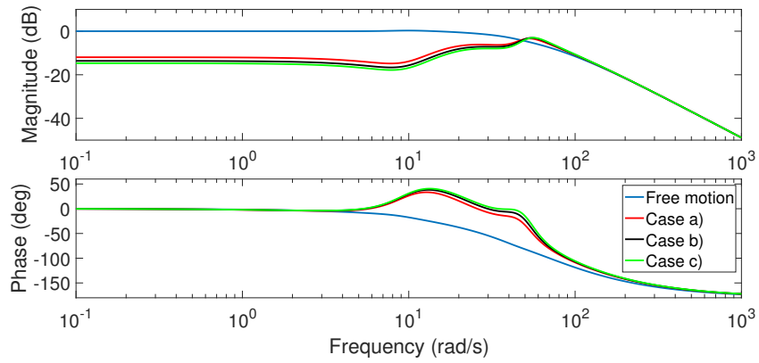
Figure 11: Bode diagrams of the closed-loop system (34) in the cases of free motion and constrained motion with the three mentioned impedances
