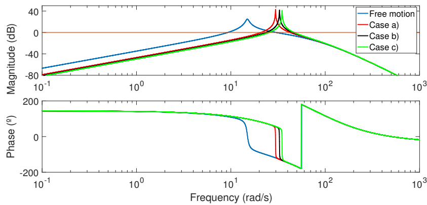
Figure 10: Bode diagrams of the open-loop system C(s)M(s)G_p(s, K, \nu) in the cases of free motion and constrained motion with the three mentioned impedances
