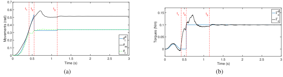
Figure 14: Results for Experiment #2: (a) angles, (b) torques
