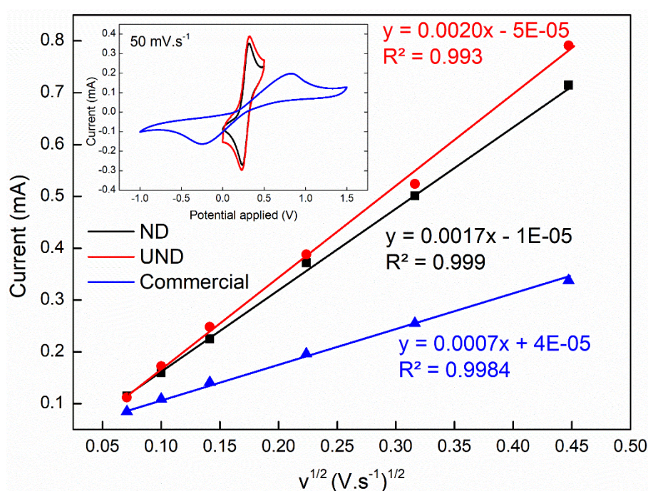
Figure 3. (A) Square root of the scan rate and the current intensity for the studied electrodes and the different CV shapes obtained for the electrodes (inset).
