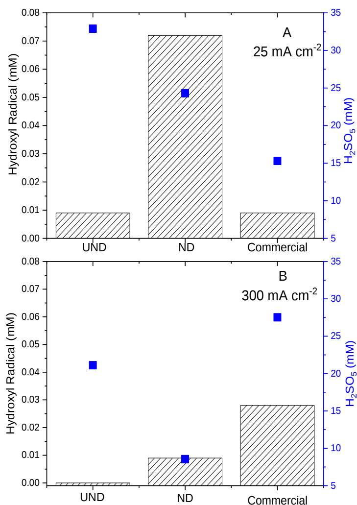
Figure 7. Hydroxyl radical and Caro's acid production for the studied electrodes in current densities 25 and 300 \text{mA cm}^{-2} .
