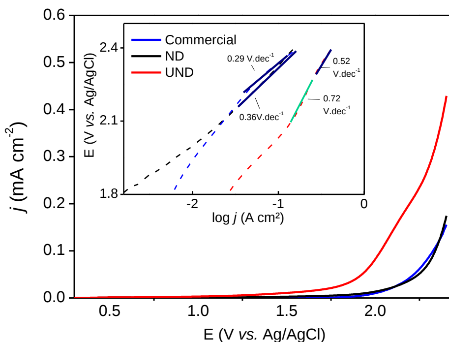
Fig 5. Polarization curves recorded for the studied electrodes in 1 M H 2 SO 4 (inset shows Tafel plots).
