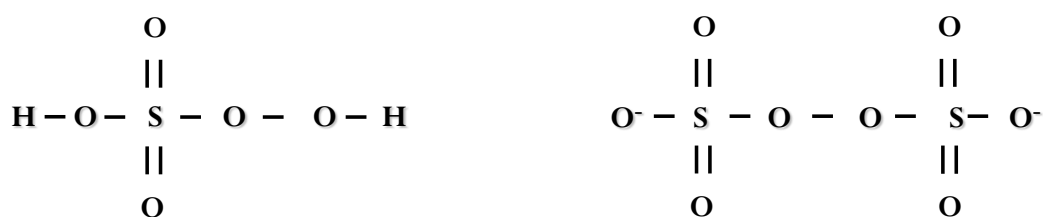
Figure 1. Molecular structure of peroxymonosulphuric acid (Caro's acid) and diperoxosulphuric acid (persulphate).
