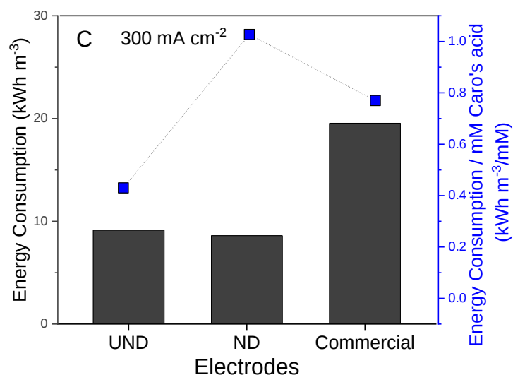
Figure 5. A) Current efficiency (%) and B) overall energy consumption and energy consumption per mM of Caro's acid at 25 mA cm -2 and C) 300 mA cm -2 for the three diamond electrodes.
