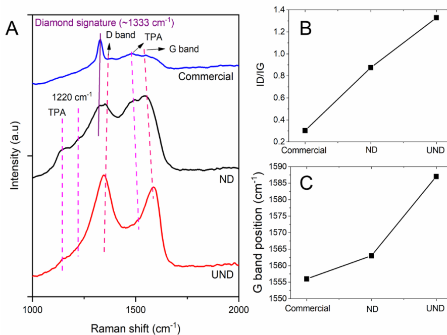
Figure 2. A) Raman spectra, B) ID/IG and C) G band position for commercial, ND and UND electrodes.
