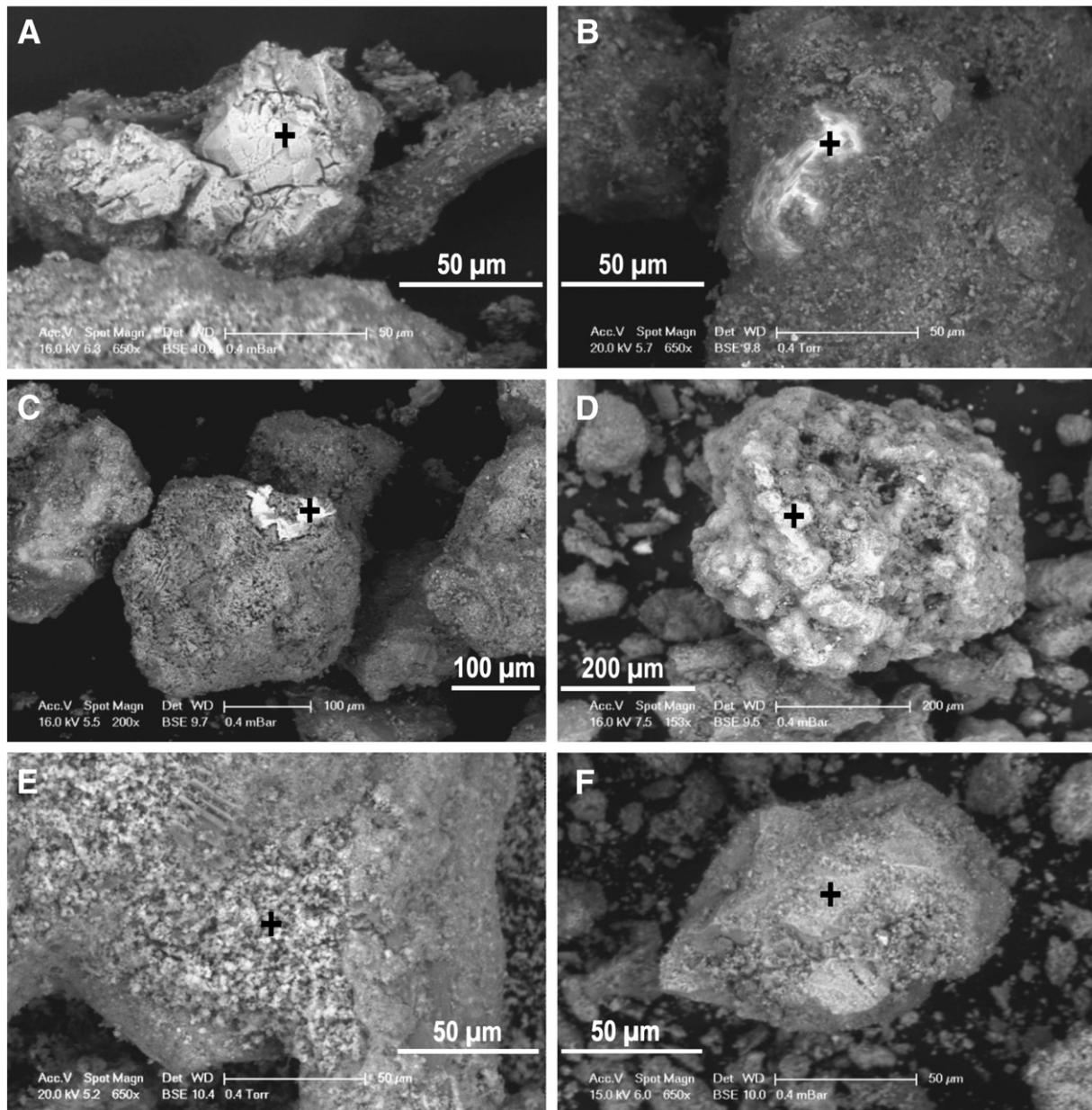
Fig. 7. BSE images of mineral grains from samples of tailings (TA) and calcines (CA). A: SC-10, pyrite (TA); Acc. V: 16 kV. B: SC-9, galena (TA); Acc. V: 20 kV. C: SC-10, sphalerite (TA); Acc. V: 16 kV. D: SC-10, Zn-Fe sulphate (TA); Acc. V: 16 kV. E: SC-5, As bearing goethite-like grain (TA); Acc. V: 20 kV. F: SC-12, As bearing goethite-like grain (CA); Acc. V: 15 kV. The cross (+) indicates EDX point analysis.
